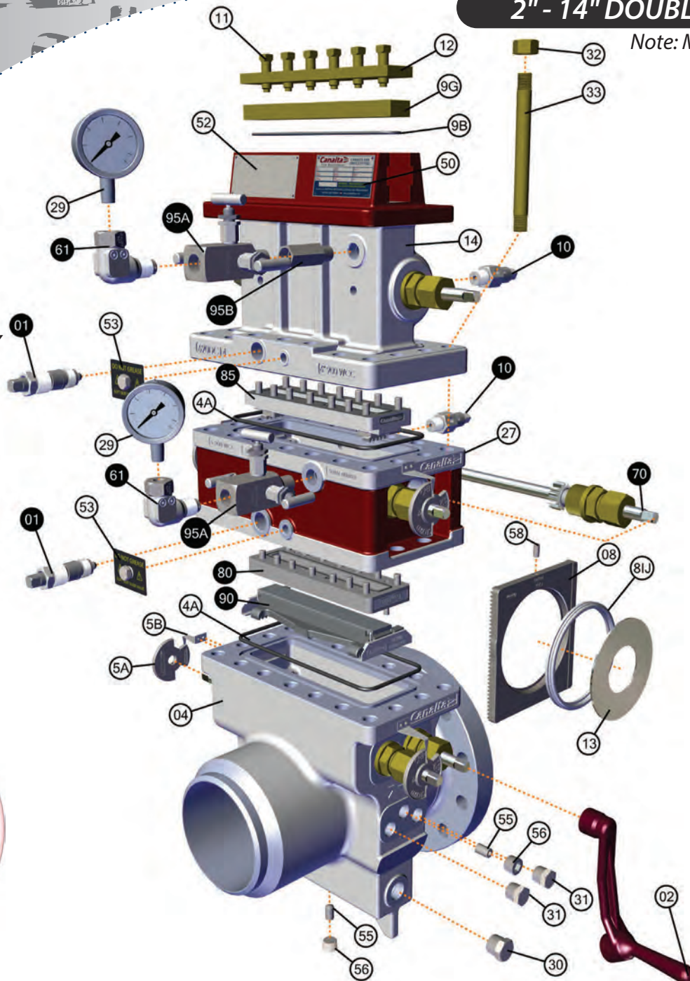
01 - EQUALIZER ASSEMBLY
