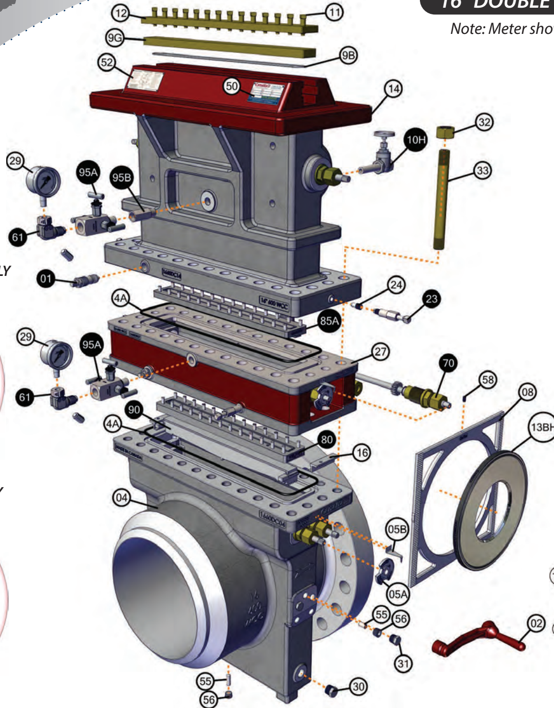
90 - VALVE ASSEMBLY
