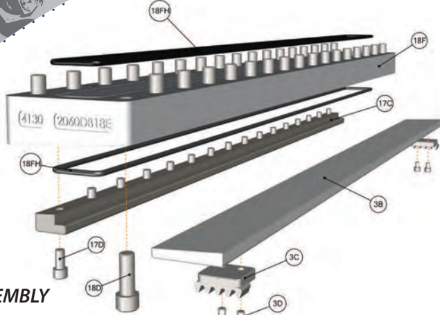
85 - WEDGE VALVE SEAT ASSEMBLY
