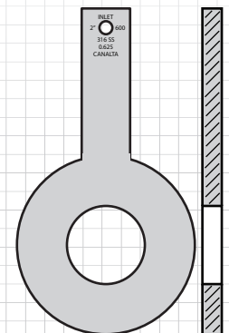
Concentric Restriction Plate
