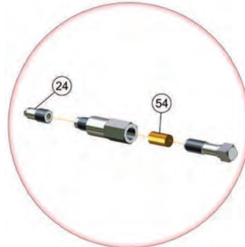
23 - GREASE GUN ASSEMBLY (Used only on Grease Type Seat)
