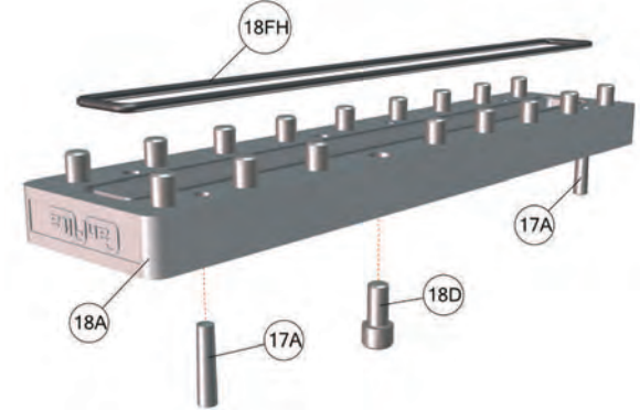
90 - VALVE ASSEMBLY
