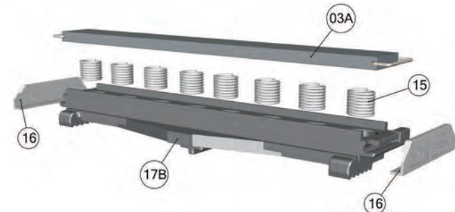
90 - CLIPPER VALVE ASSEMBLY
